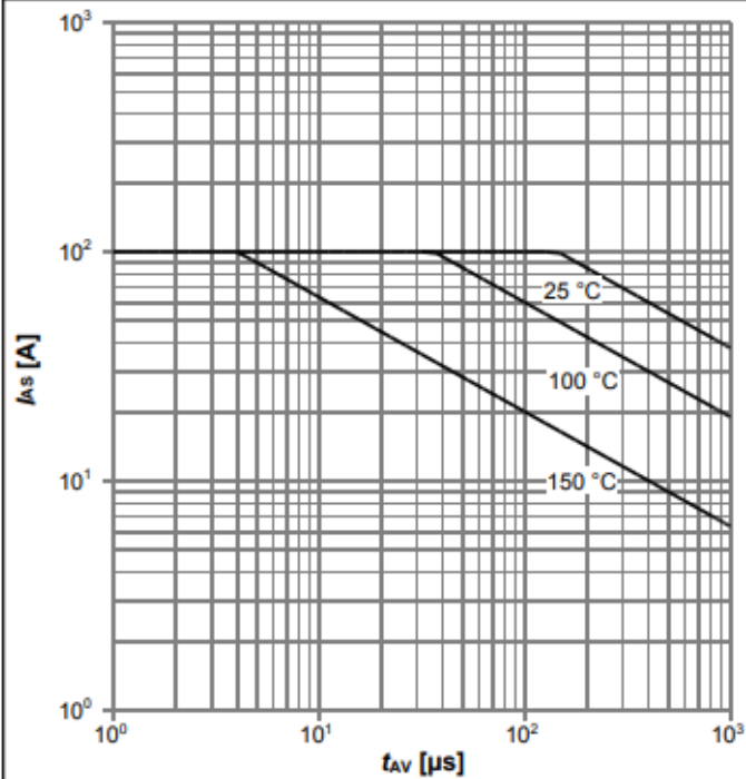
Diagram 13: Avalanche characteristics
