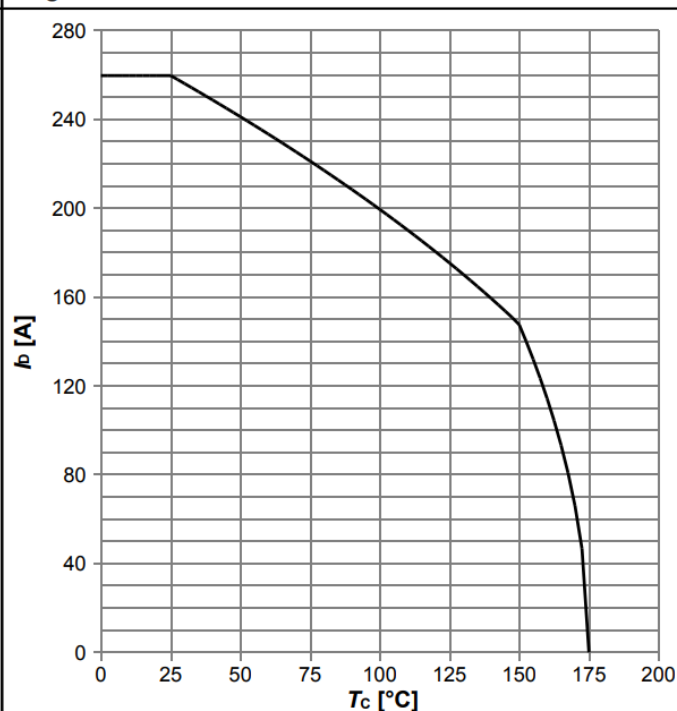
Diagram 2: Drain current
