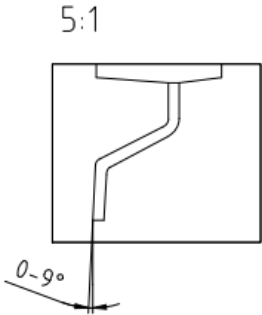
PG-TO263-3-10: OPTIONAL
