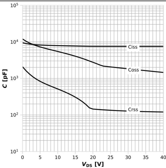
Diagram 11: Typ. capacitances
