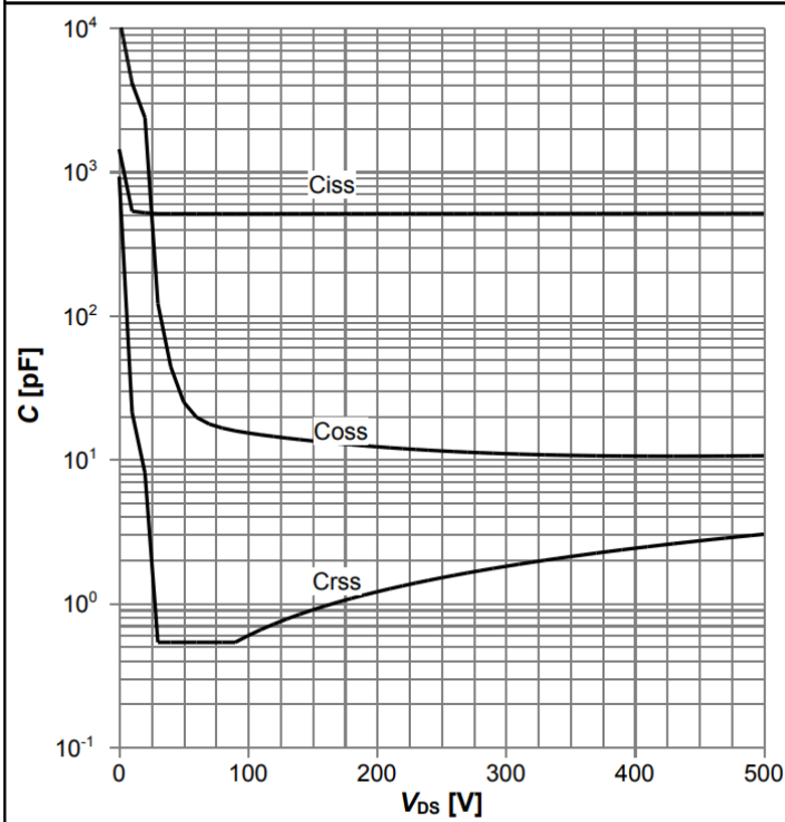
Diagram 14: Typ. capacitances
