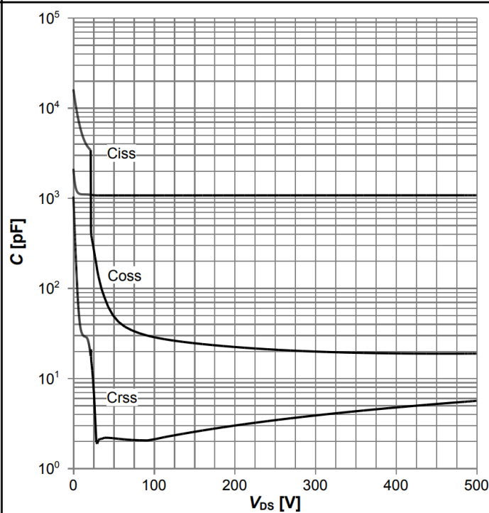
Diagram 14: Typ. capacitances
