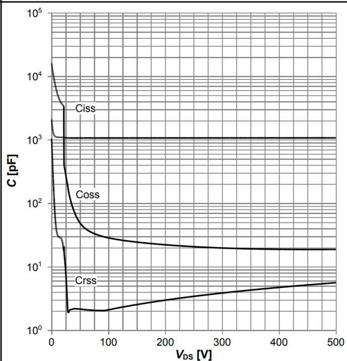
Diagram 14: Typ. capacitances
