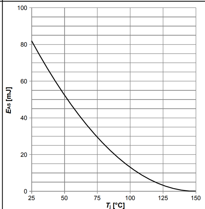
Diagram 12: Avalanche energy
