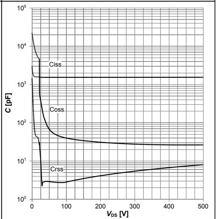
Diagram 14: Typ. capacitances
