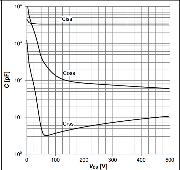
Diagram 18: Typ. capacitances
