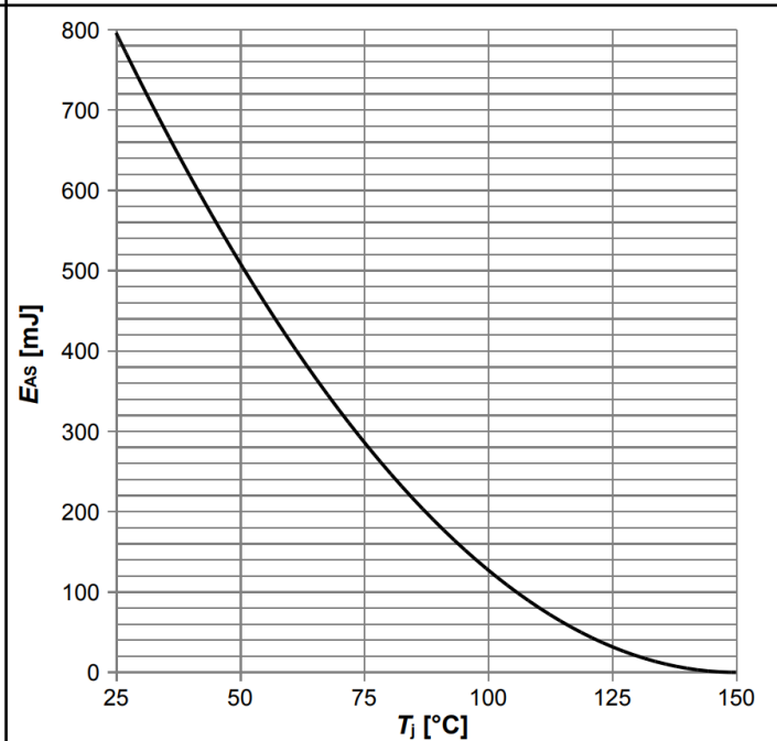
Diagram 16: Avalanche energy
