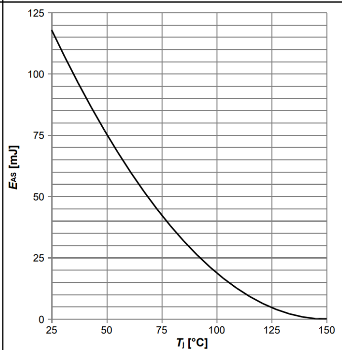
Diagram 12: Avalanche energy
