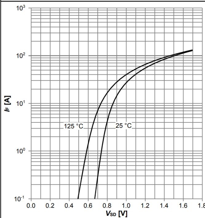
Diagram 11: Forward characteristics of reverse diode
