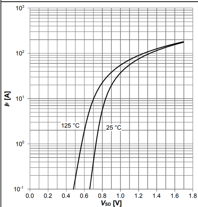
Diagram 11: Forward characteristics of reverse diode
