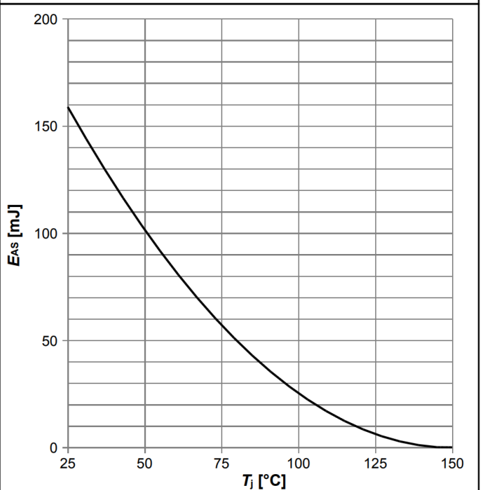
Diagram 12: Avalanche energy
