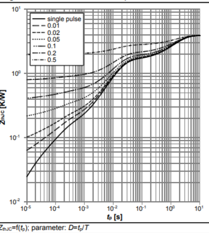
Diagram 4: Max. transient thermal impedance
