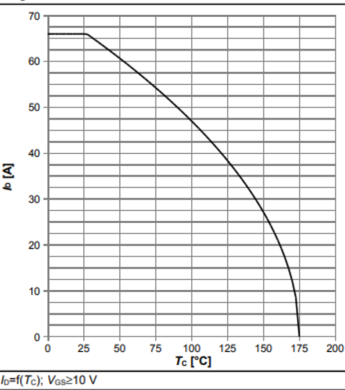
Diagram 2: Drain current
