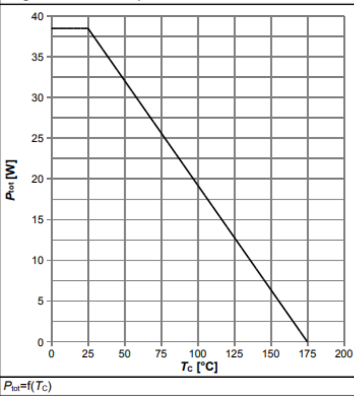
Diagram 1: Power dissipation
