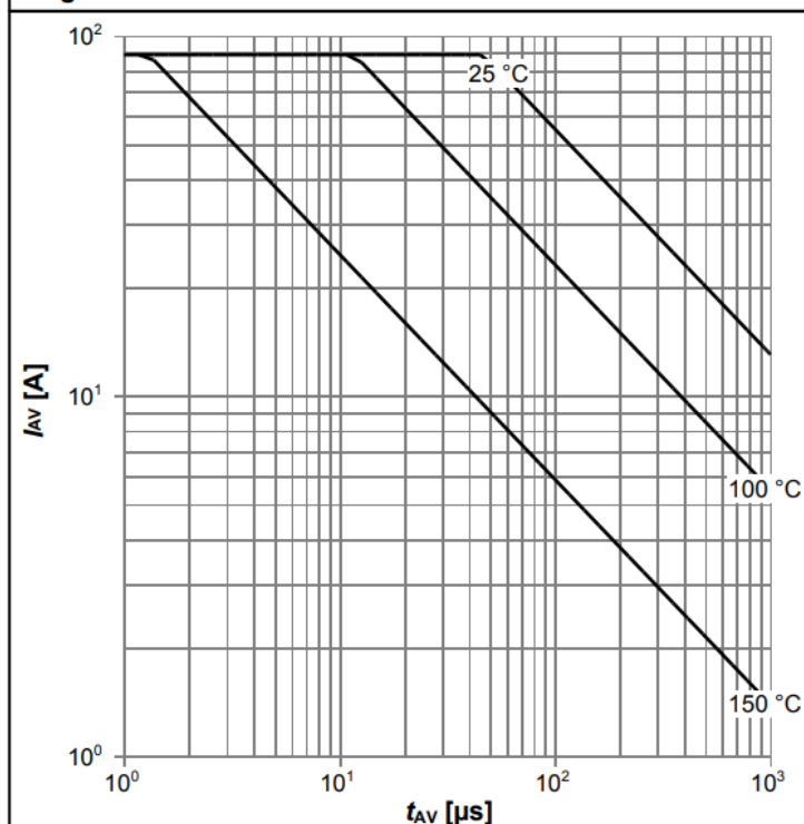
Diagram 13: Avalanche characteristics
