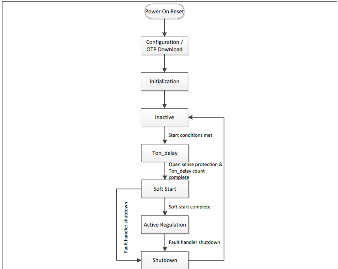
Figure 14 State Diagram
