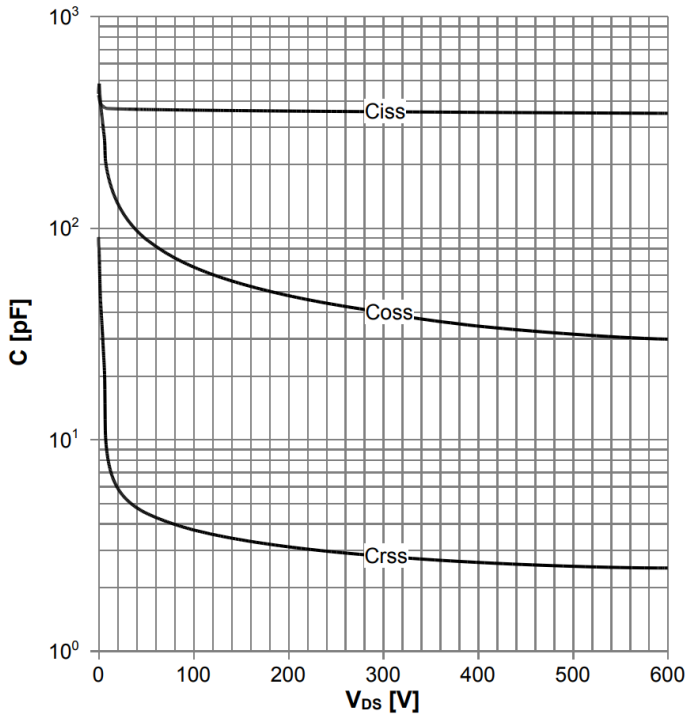
Diagram 15: Typ. capacitances
