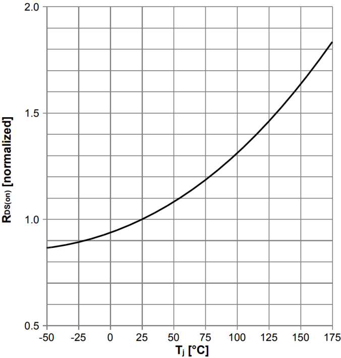
Diagram 8: Drain-source on-state resistance
