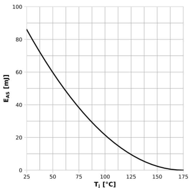
Diagram 13: Avalanche energy
