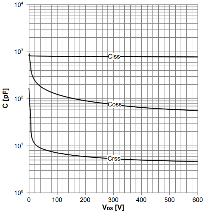
Diagram 15: Typ. capacitances
