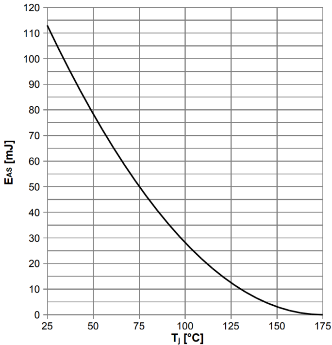
Diagram 13: Avalanche energy
