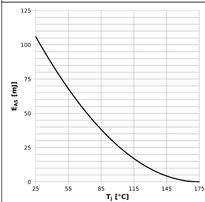
Diagram 13: Avalanche energy
