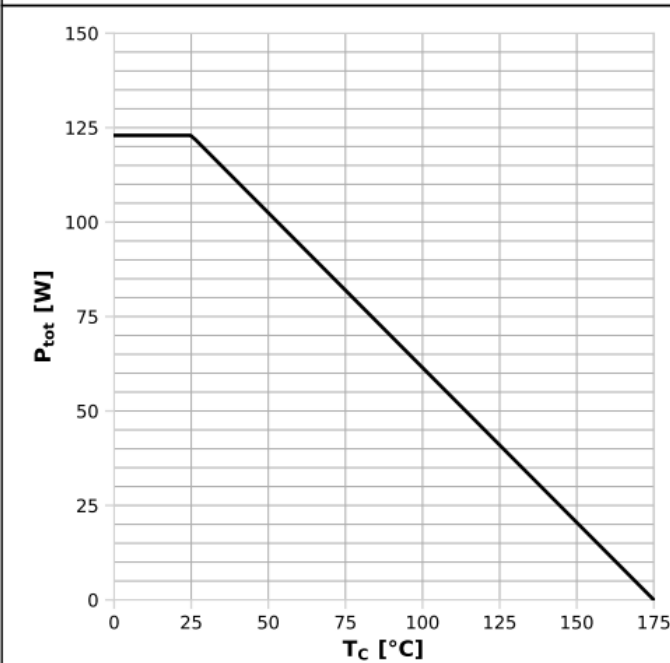
Diagram 1: Power dissipation
