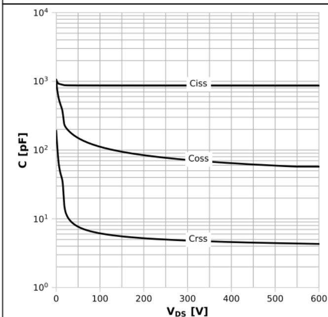
Diagram 15: Typ. capacitances
