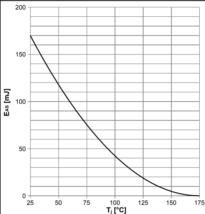
Diagram 13: Avalanche energy
