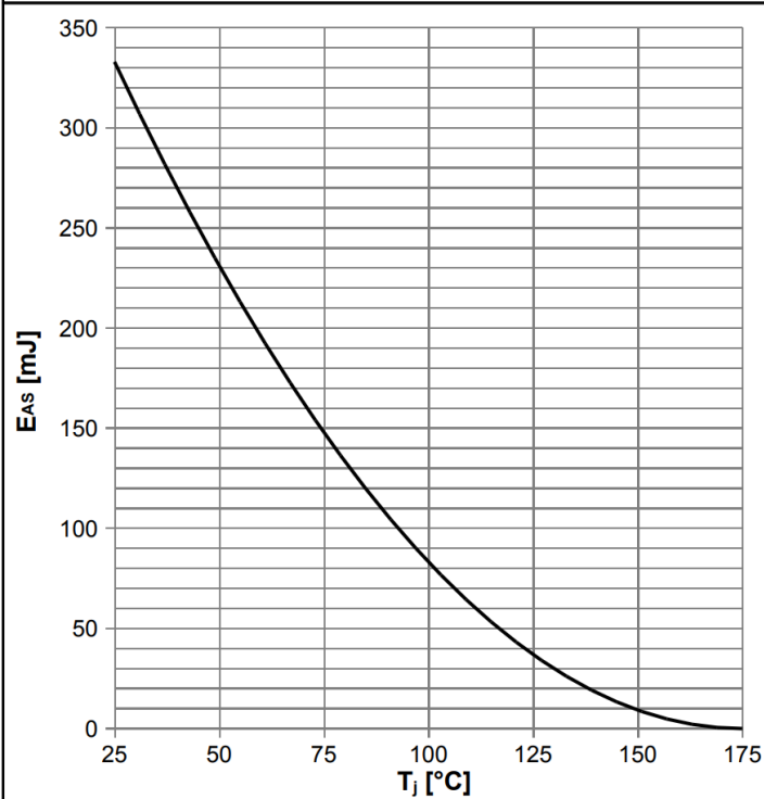
Diagram 13: Avalanche energy
