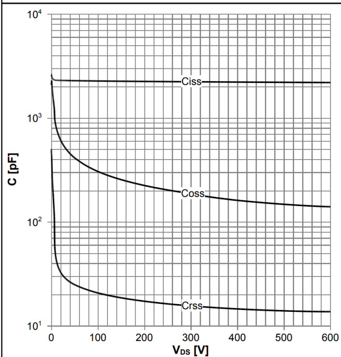
Diagram 15: Typ. capacitances
