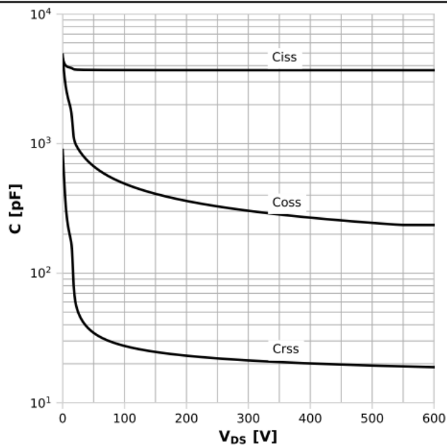
Diagram 15: Typ. capacitances
