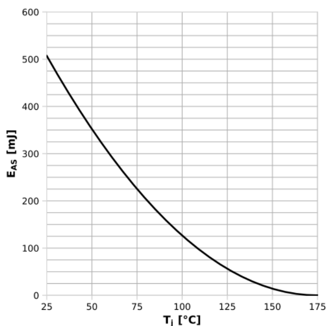
Diagram 13: Avalanche energy
