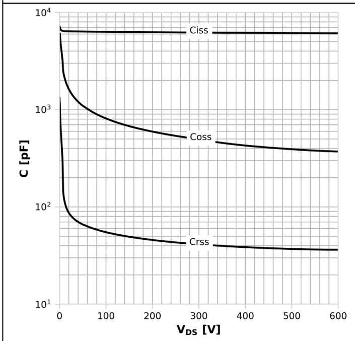
Diagram 15: Typ. capacitances
