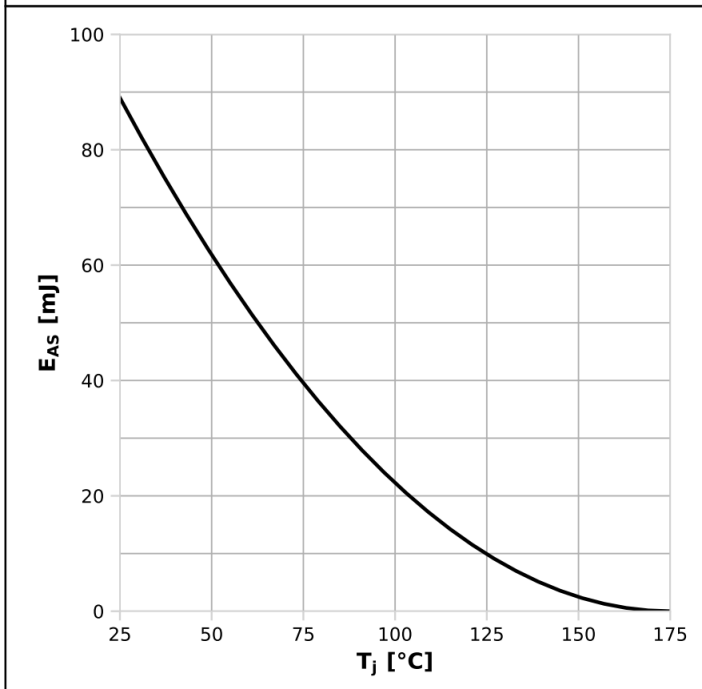
Diagram 13: Avalanche energy
