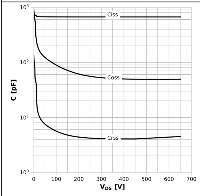
Diagram 15: Typ. capacitances
