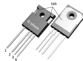
PG-TO247-4
