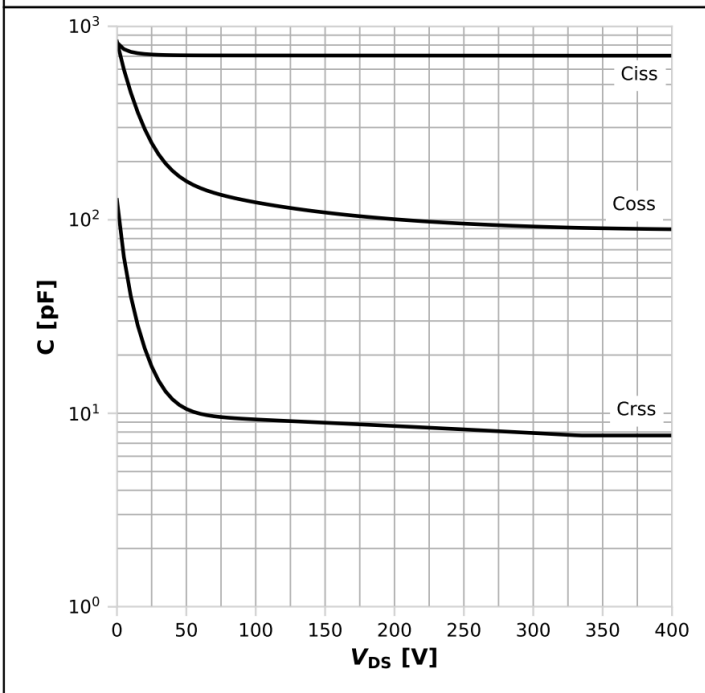
Diagram 15: Typ. capacitances
