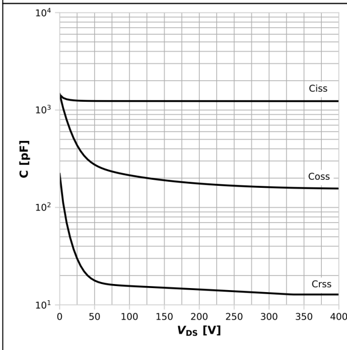
Diagram 15: Typ. capacitances
