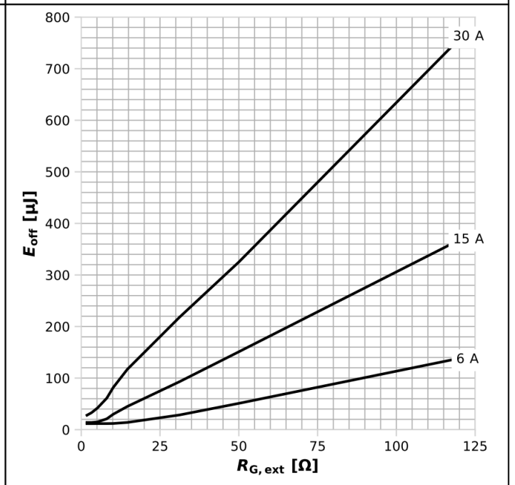
Diagram 24: Typ. turn-off switching losses
