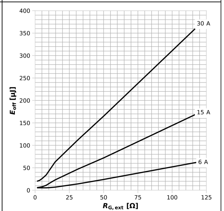
Diagram 22: Typ. turn-off switching losses
