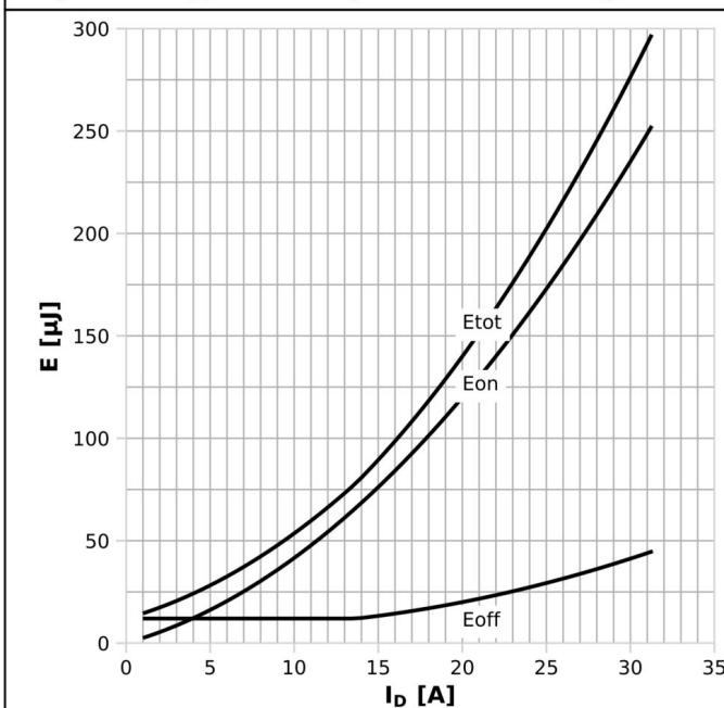
Diagram 19: Typ. Switching Losses vs switching current
