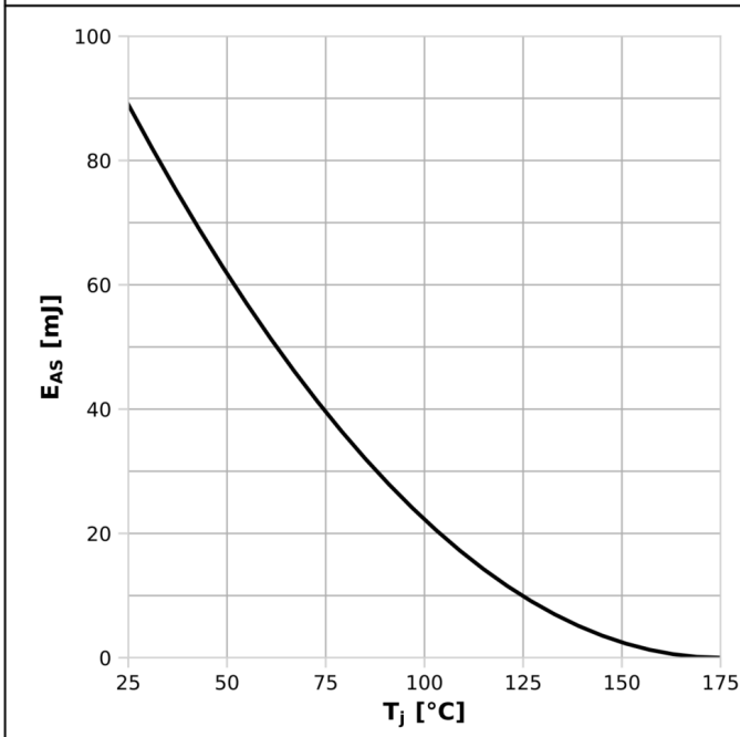
Diagram 13: Avalanche energy
