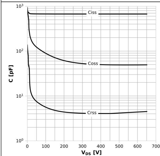
Diagram 15: Typ. capacitances
