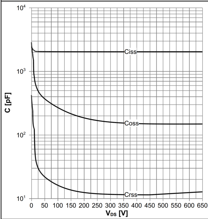
Diagram 15: Typ. capacitances
