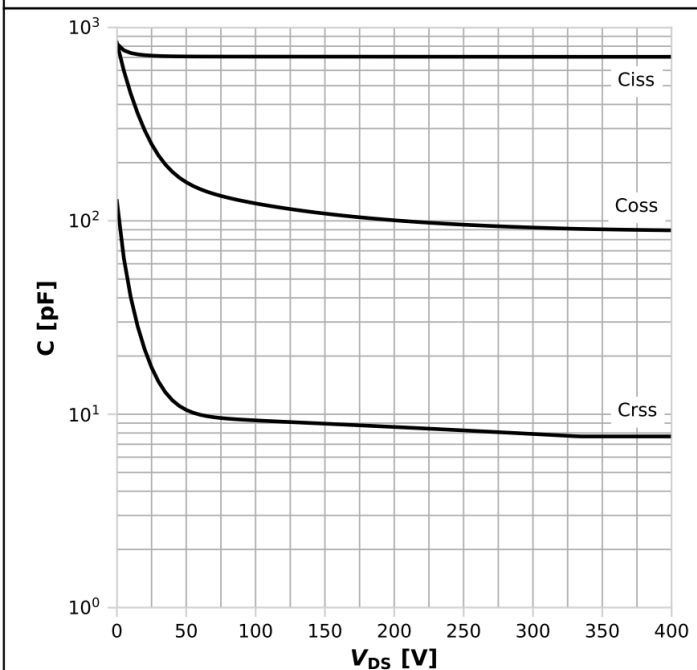
Diagram 15: Typ. capacitances
