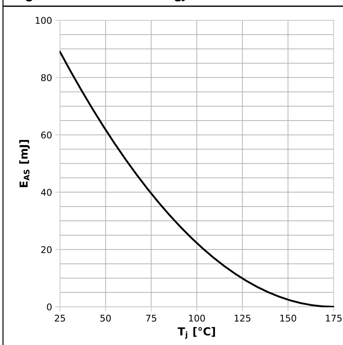
Diagram 13: Avalanche energy
