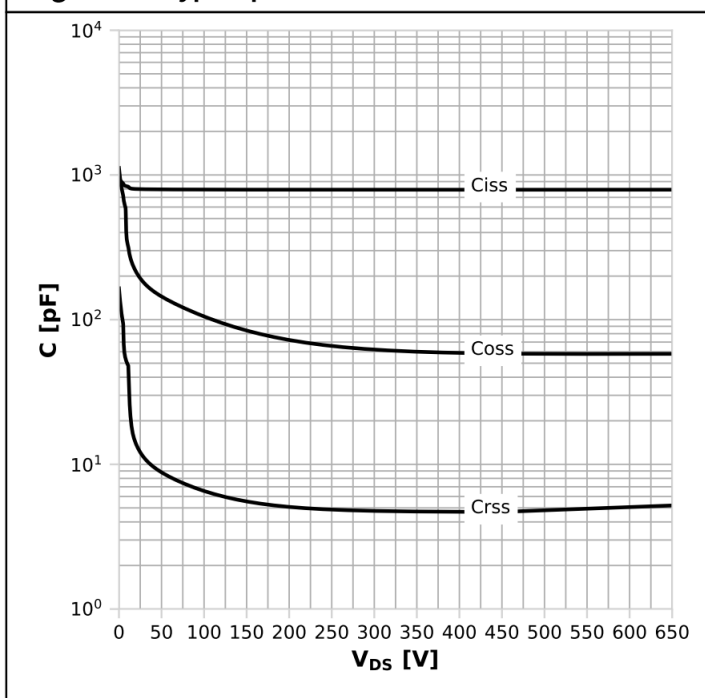
Diagram 15: Typ. capacitances
