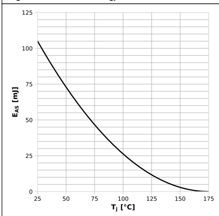
Diagram 13: Avalanche energy
