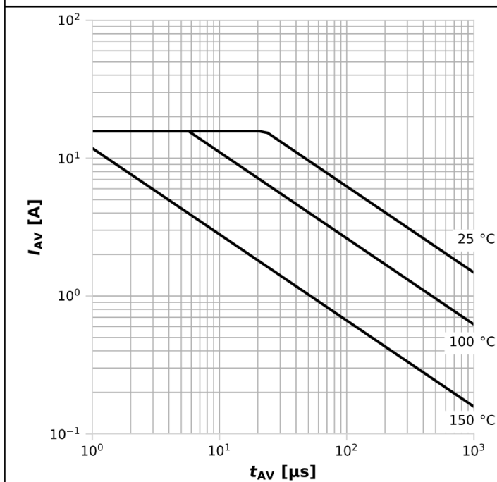
Diagram 19: Avalanche characteristics
