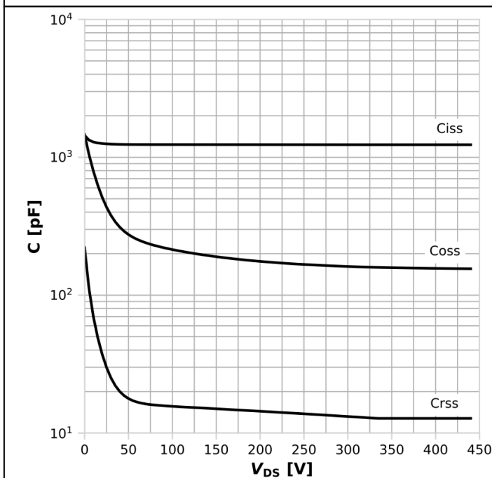
Diagram 15: Typ. capacitances
