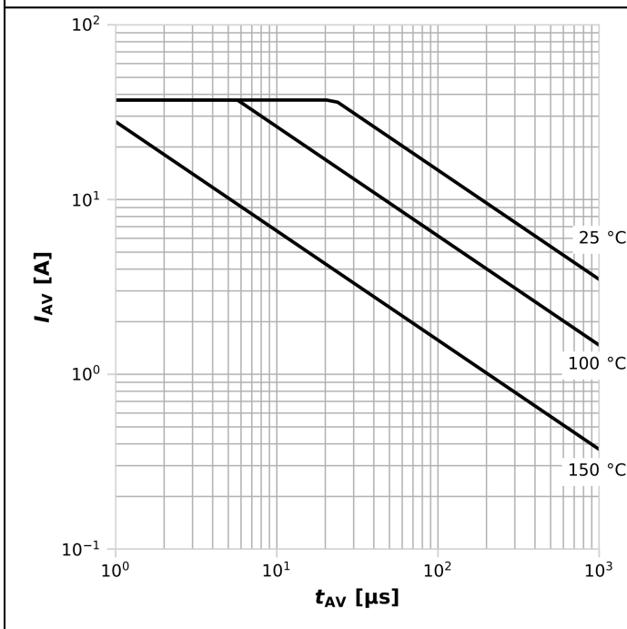
Diagram 19: Avalanche characteristics
