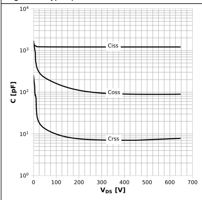
Diagram 15: Typ. capacitances
