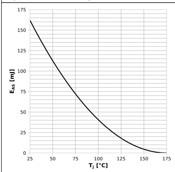
Diagram 13: Avalanche energy
