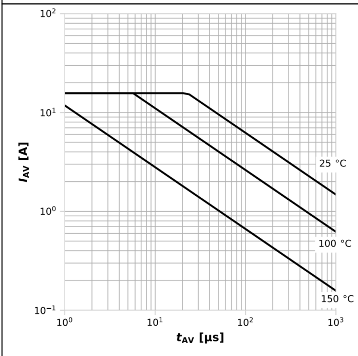
Diagram 19: Avalanche characteristics
