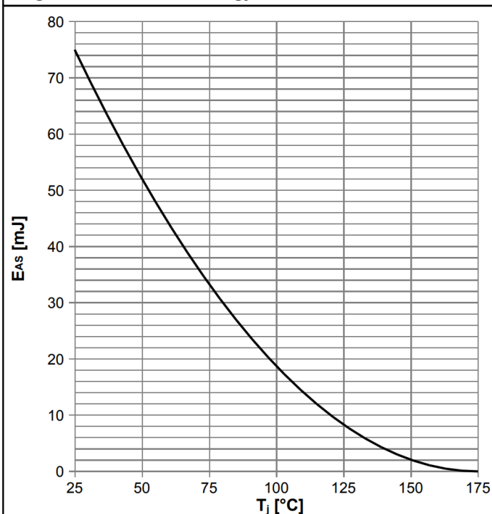
Diagram 13: Avalanche energy
