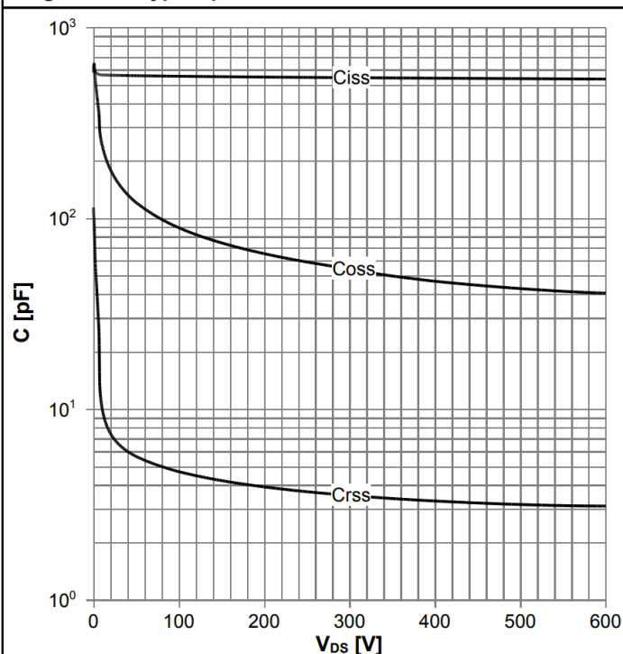
Diagram 15: Typ. capacitances
