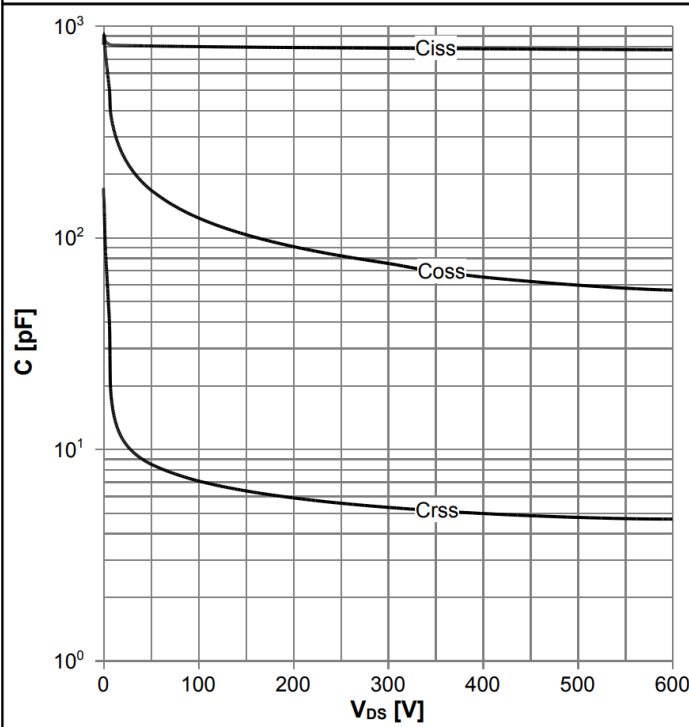
Diagram 15: Typ. capacitances
