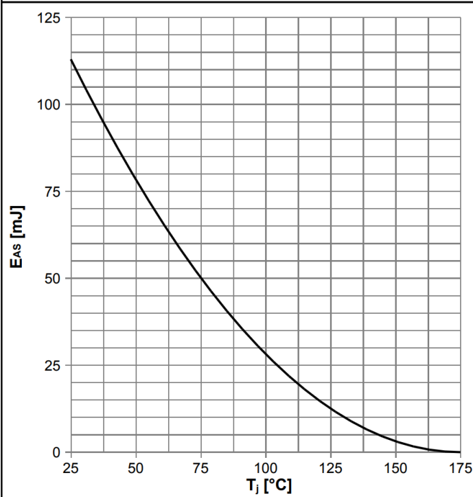
Diagram 13: Avalanche energy
