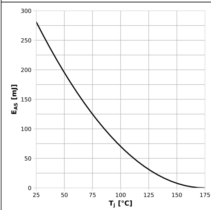
Diagram 13: Avalanche energy
