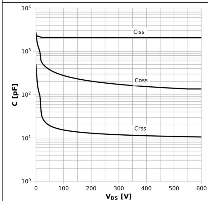
Diagram 15: Typ. capacitances
