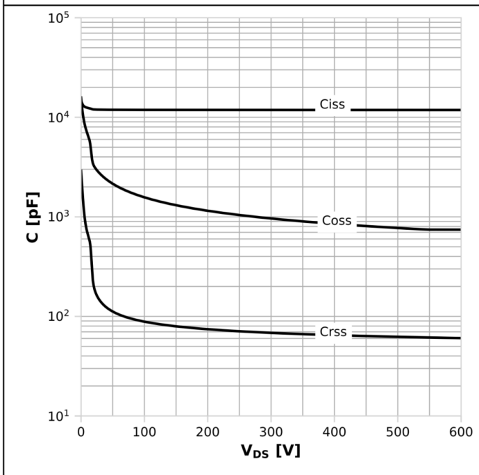
Diagram 15: Typ. capacitances
