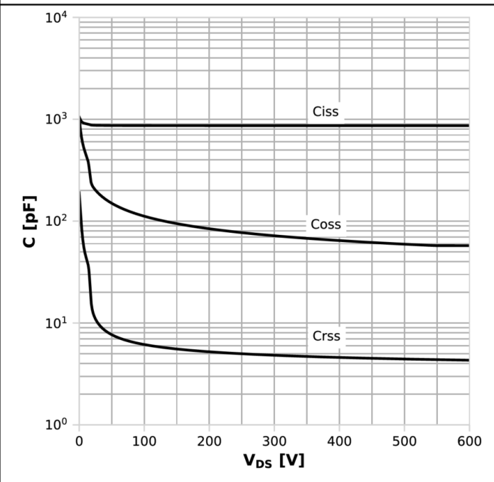
Diagram 15: Typ. capacitances
