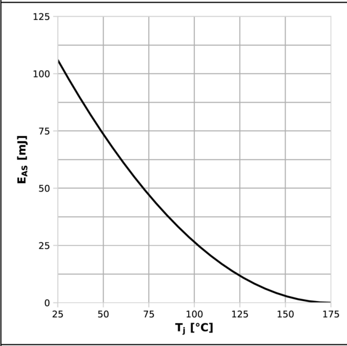
Diagram 13: Avalanche energy
