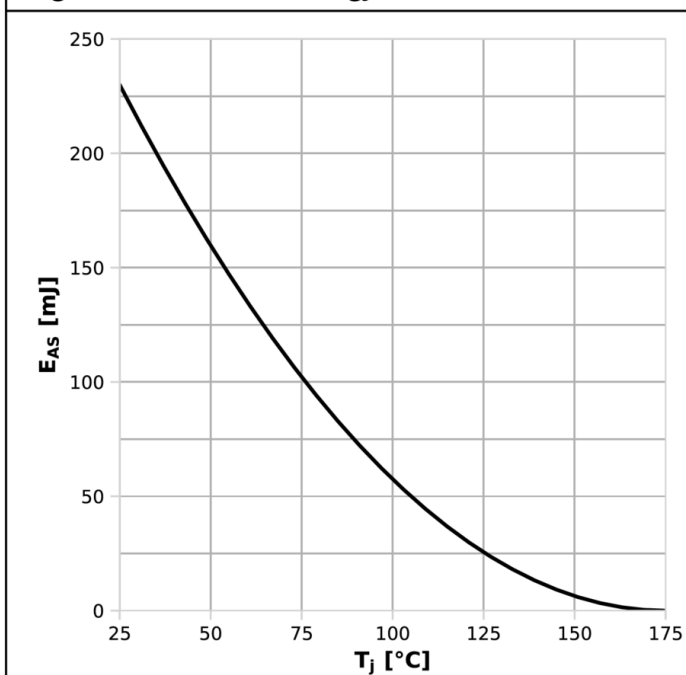
Diagram 13: Avalanche energy
