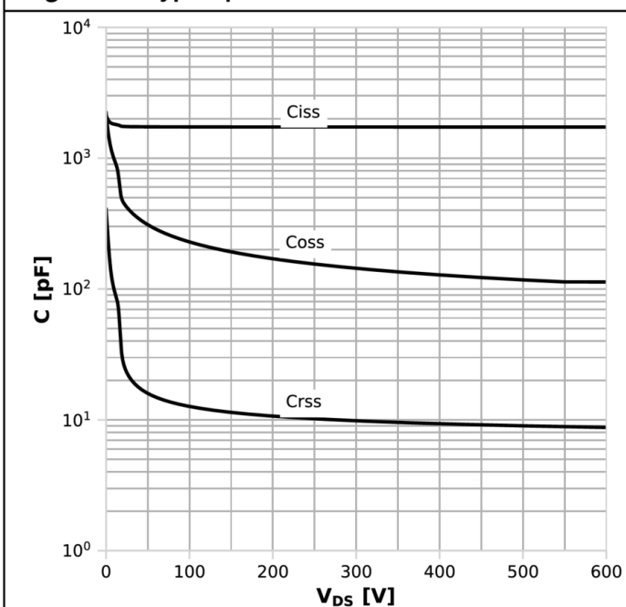
Diagram 15: Typ. capacitances
