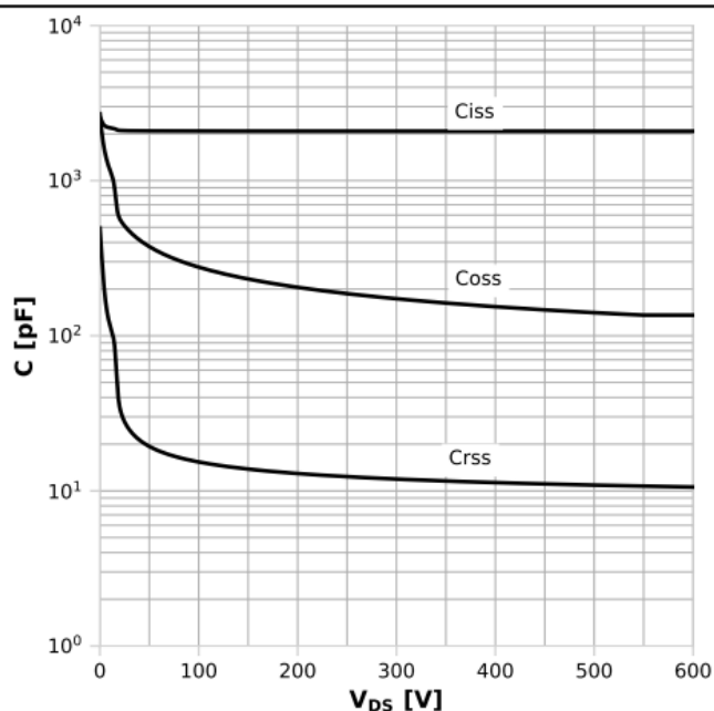
Diagram 15: Typ. capacitances
