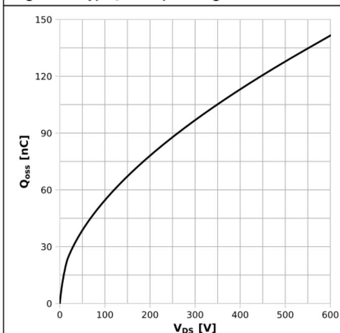
Diagram 17: Typ. Qoss output charge
