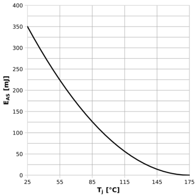
Diagram 13: Avalanche energy
