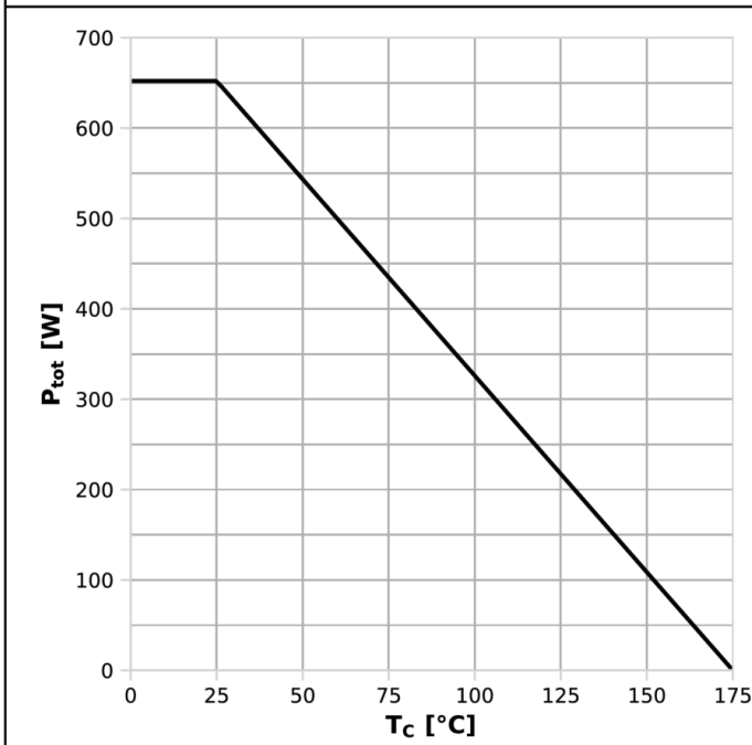
Diagram 1: Power dissipation
