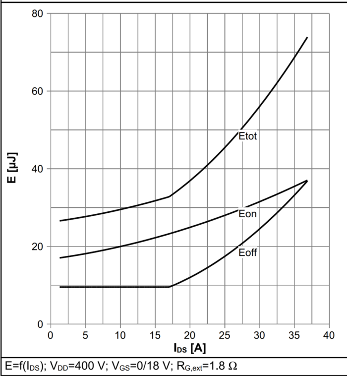
Diagram 19: Typ. Switching Losses vs switching current
