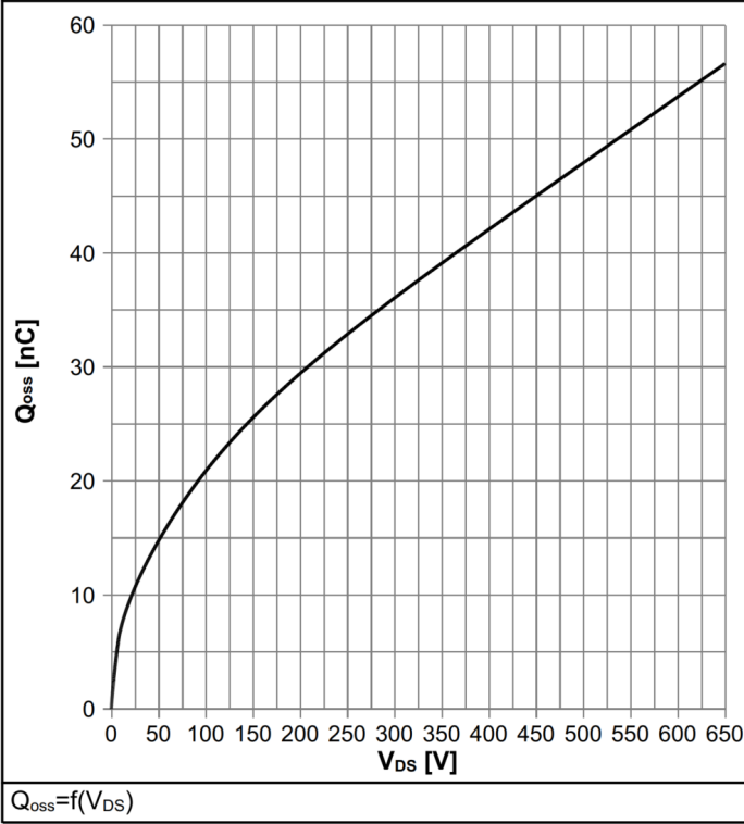
Diagram 17: Typ. Qoss output charge
