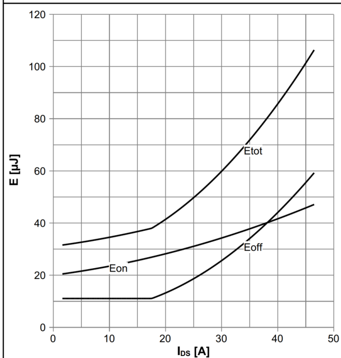
Diagram 19: Typ. Switching Losses vs switching current
