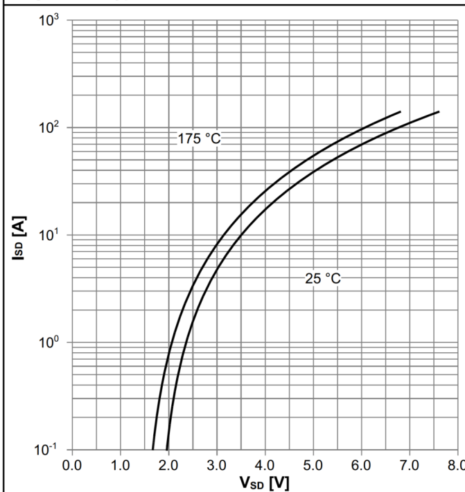
Diagram 11: Typ. reverse drain current characteristics
