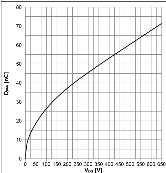
Diagram 17: Typ. Qoss output charge
