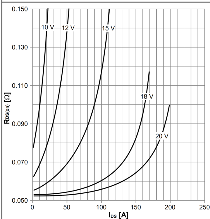
Diagram 7: Typ. drain-source on-state resistance
