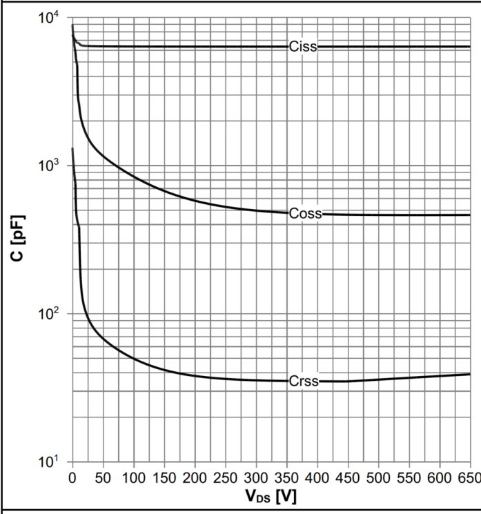
Diagram 15: Typ. capacitances
