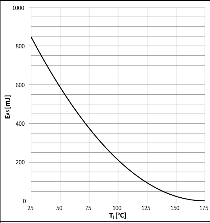
Diagram 13: Avalanche energy
