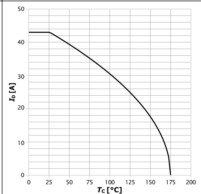
Diagram 2: Drain current
