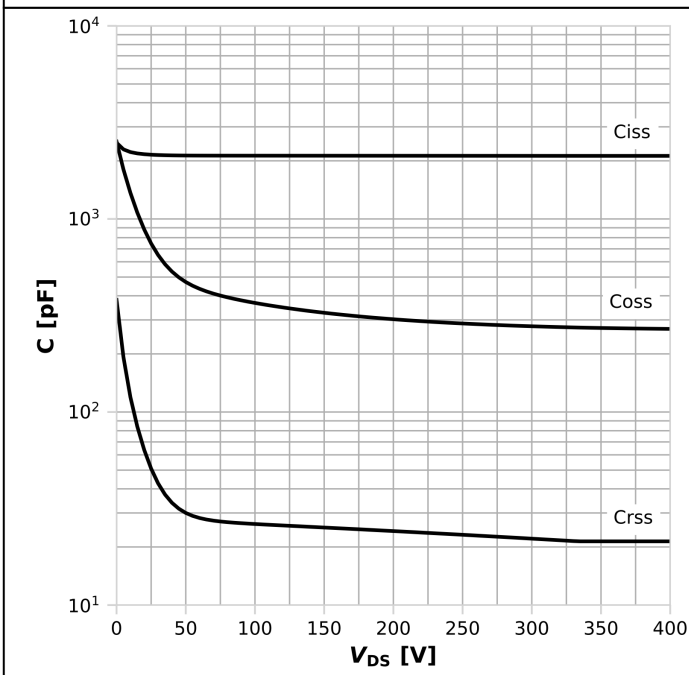
Diagram 15: Typ. capacitances
