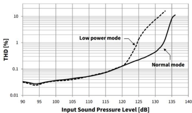
Figure 6 Typical THD vs SPL
