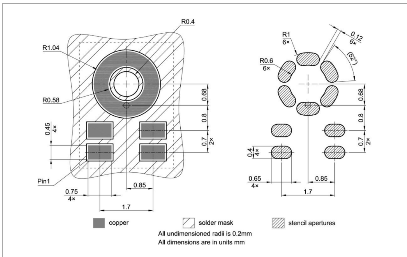
Figure 13 IM73A135V01 footprint and stencil recommendation
