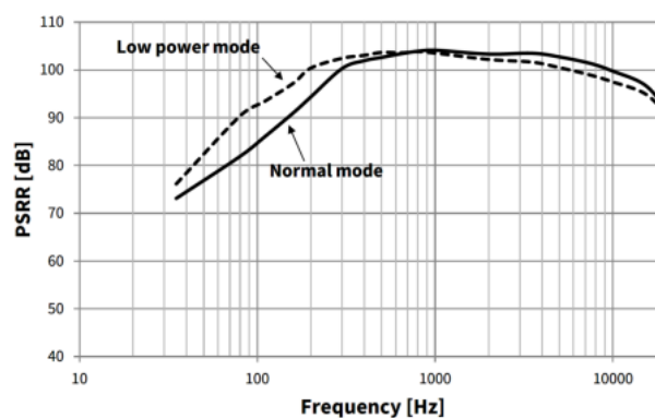
Figure 9 Typical PSRR
