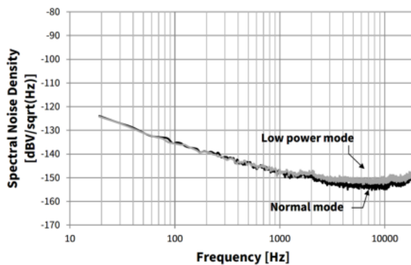
Figure 5 Typical noise floor (unweighted)
