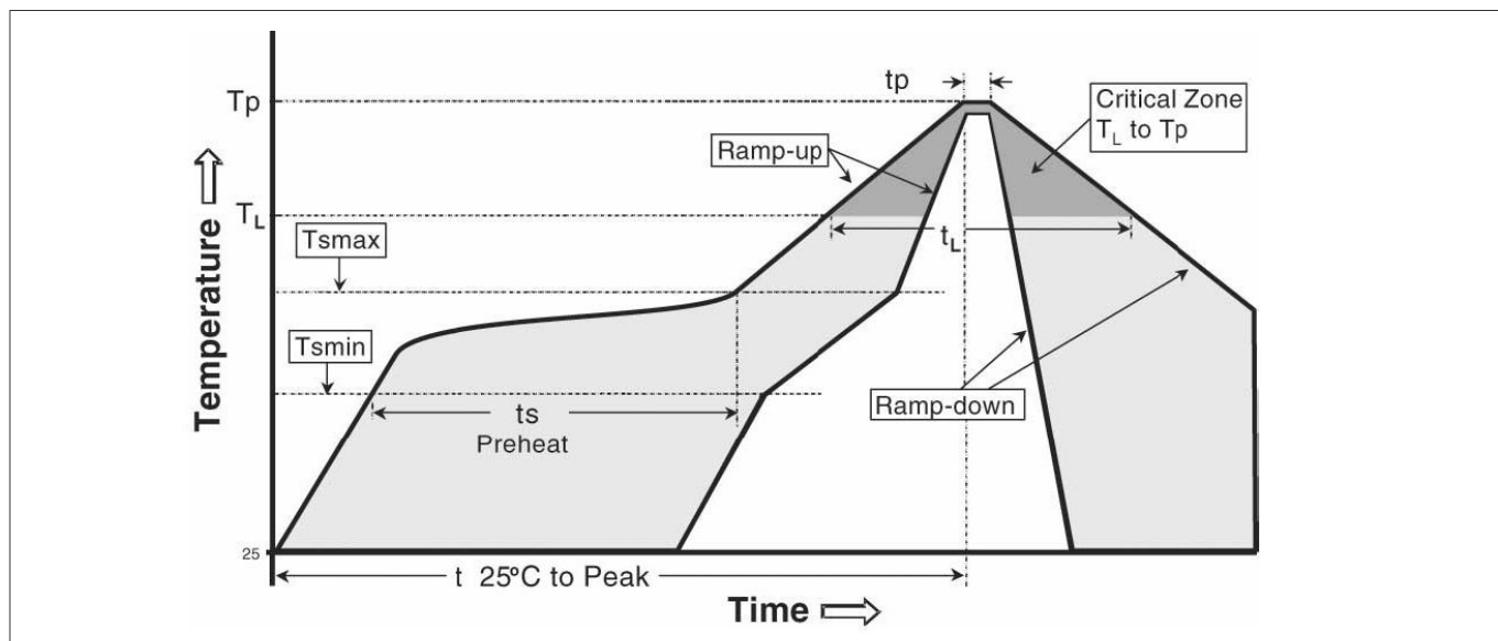
Figure 15 Recommended reflow
