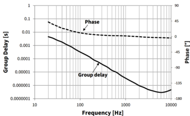
Figure 4 Typical group delay and phase response
