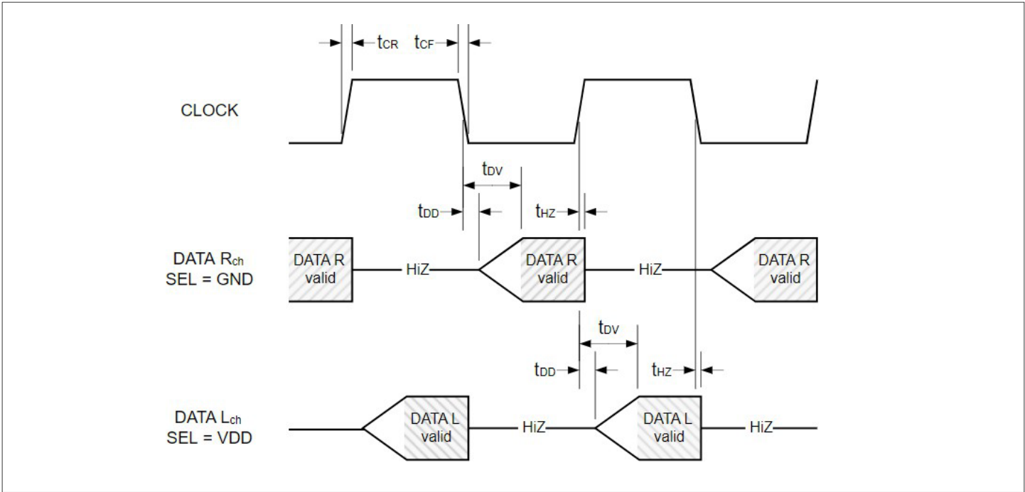
Figure 11 Timing diagram
