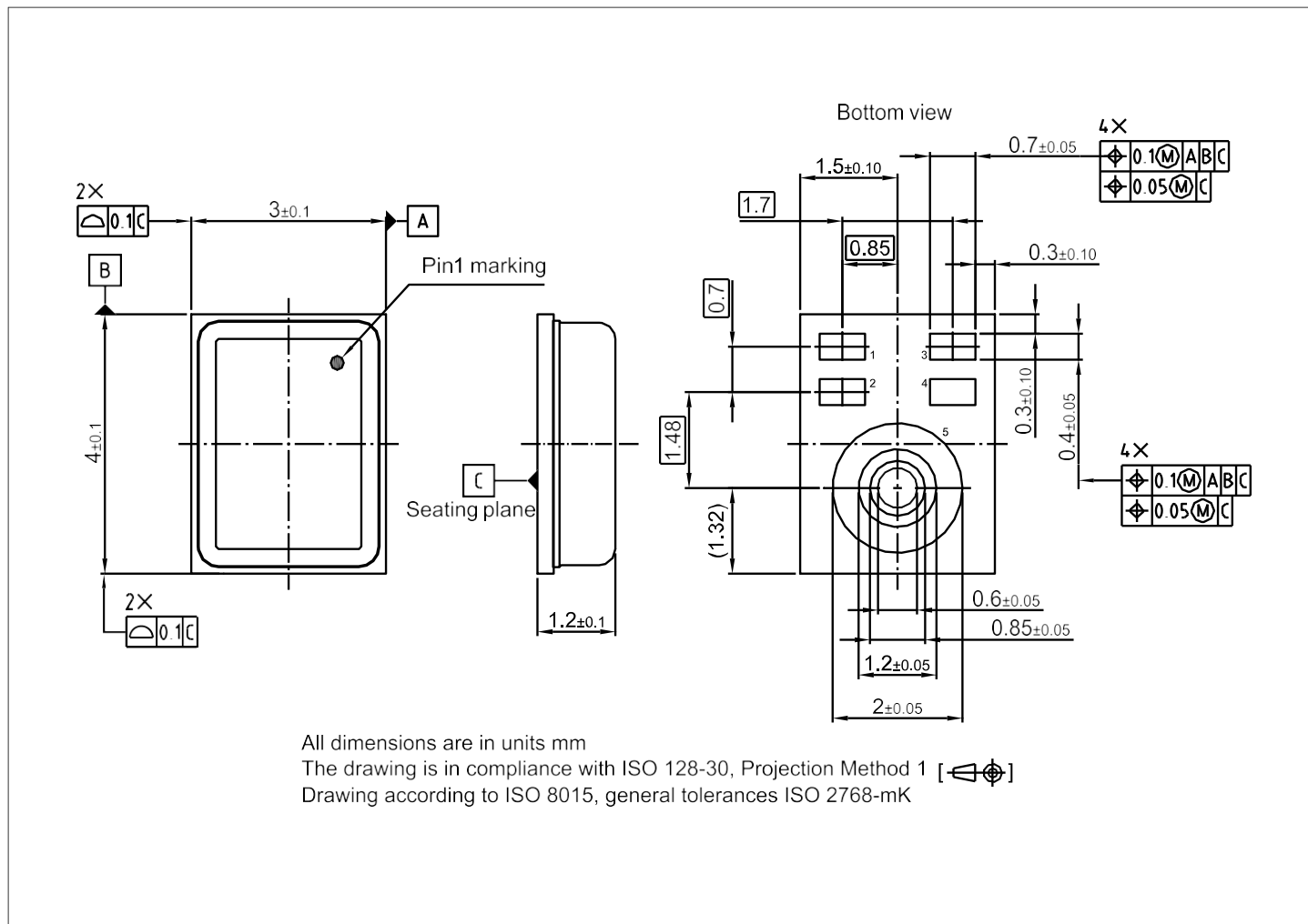
Figure 13 IM72D128VV01 package
