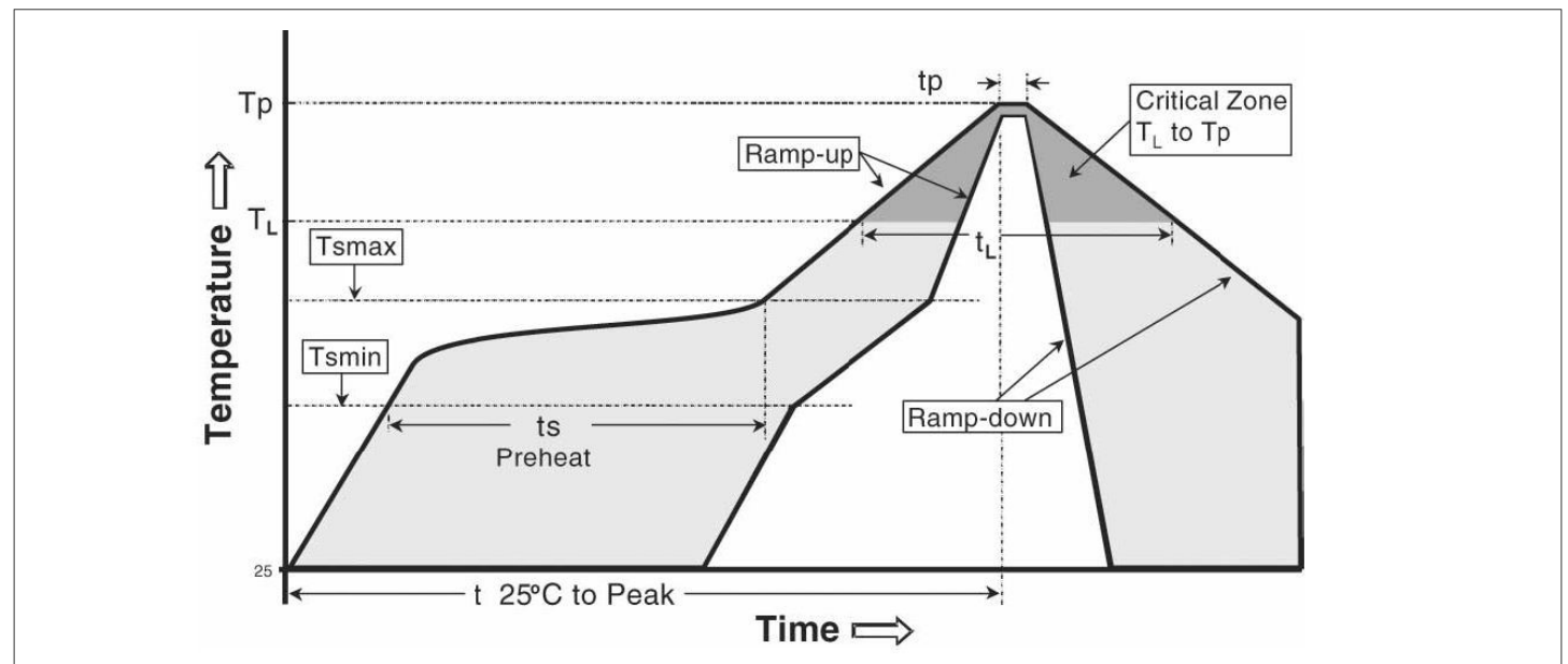
Figure 16 Recommended reflow
